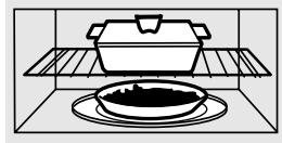
2-level reheating
