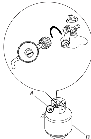
A. 20 lb LP gas fuel tank B. Gas pressure regulator/hose assembly
