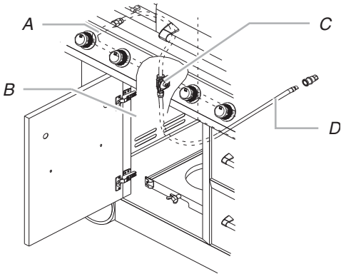
A. Manifold B. Left side panel C. Natural gas pressure regulator/hose assembly D. 10 ft (3.0 m) PVC gas hose
