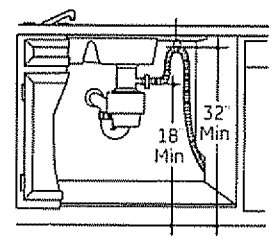
Disposer Installation
