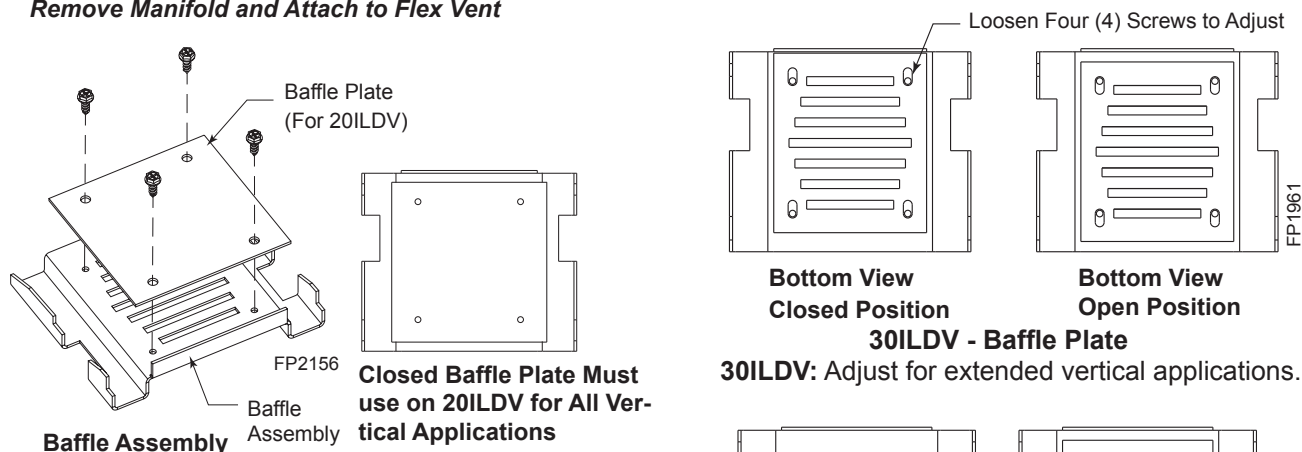
Figure 10 - Baffle Assembly and Adjustment 20ILDV Baffle Plate
