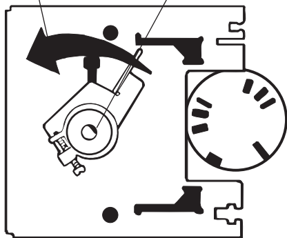
Timer-front view
