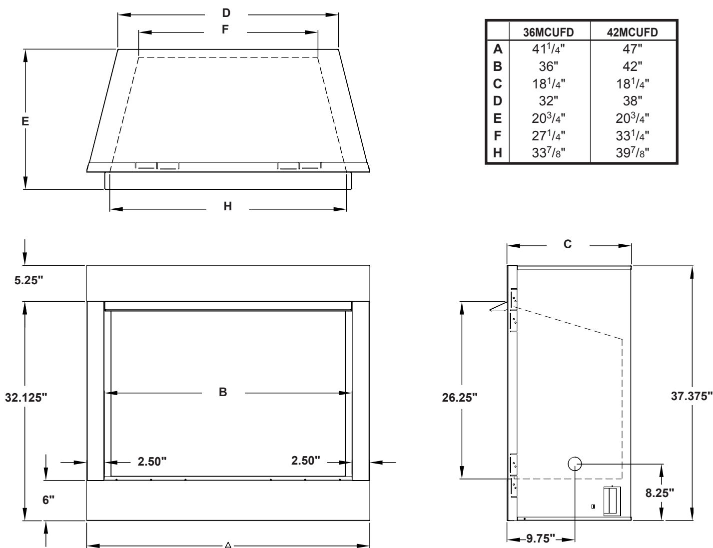
Figure 1 - Firebox Dimensions
