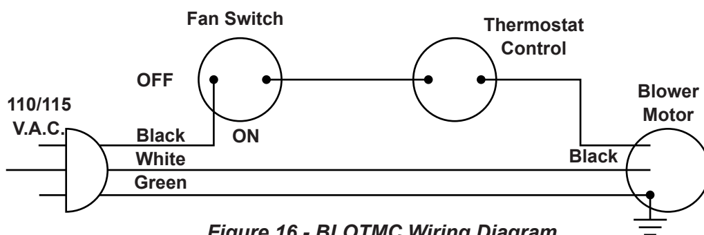
Figure 16 - BLOTMC Wiring Diagram
