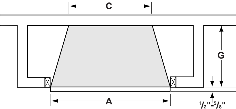
Figure 10 - Inside Chase Installation
