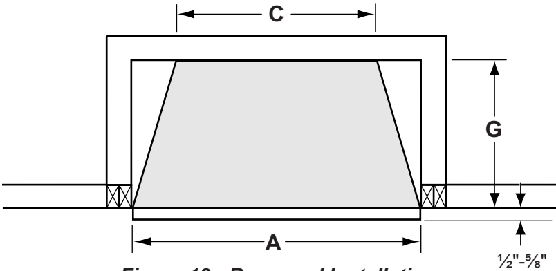
Figure 12 - Recessed Installation
