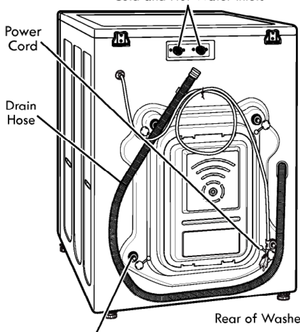
Cold and Hot Water Inlets
