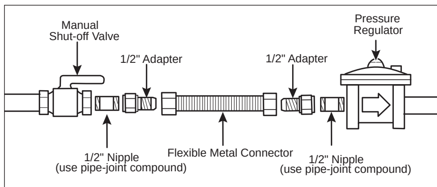
Fig. 3-2. Gas Connection
