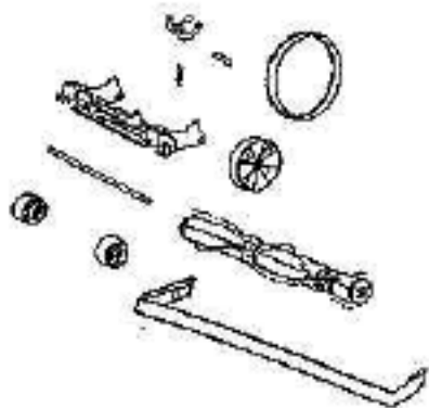
60760-3 BASE ASSY 58506-2 GASKET 54843 SPRING 14890B-119N WHEEL CARRIAGE 58206-1 WHEEL AXLE 38173-119N FRONT WHEEL 70524 GASKET 27794-119N REAR WHEEL 58814 REAR AXLE
