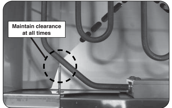
Fig. 18-2 Thermocouple clearance
