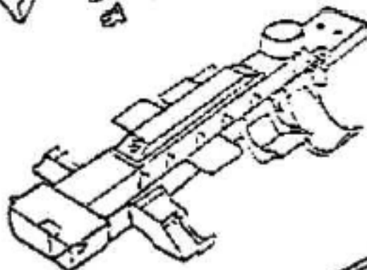
38808-1 LOWER HANDLE & MUFFLER ASSY 38398-1 ACOUSTIC PAD
