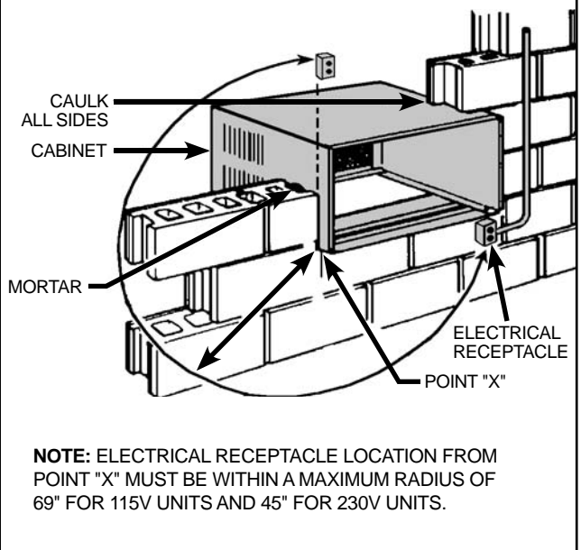
Figure E SOLID MASONRY CONSTRUCTION
