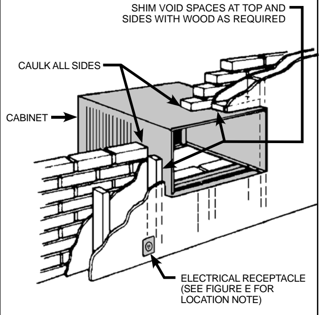
Figure D BRICK VENEER CONSTRUCTION
