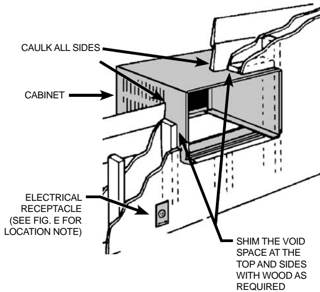
Figure C FRAME WALL CONSTRUCTION
