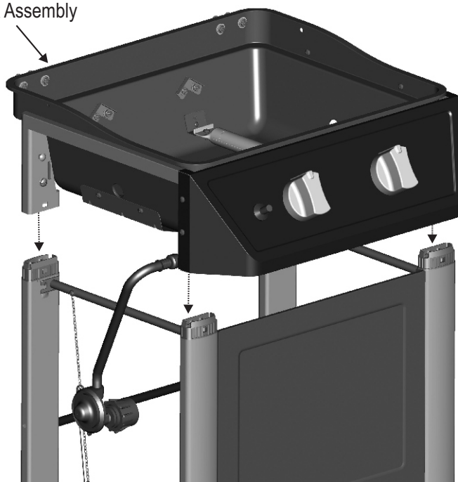
Firebox Assembly
