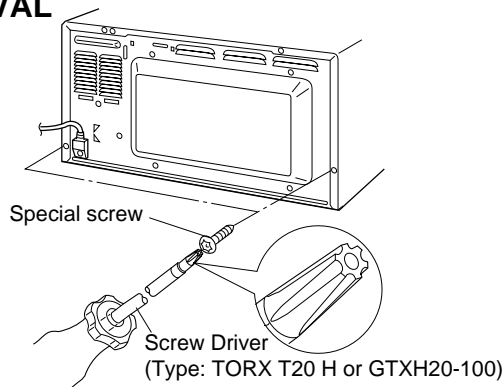
Figure C-1. Special screws position
