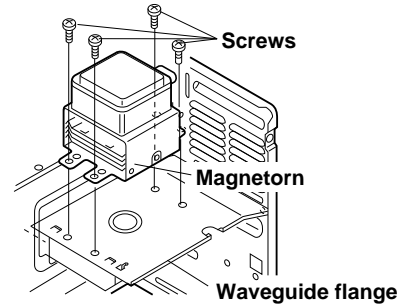
Figure C-1. Magnetron replacement
