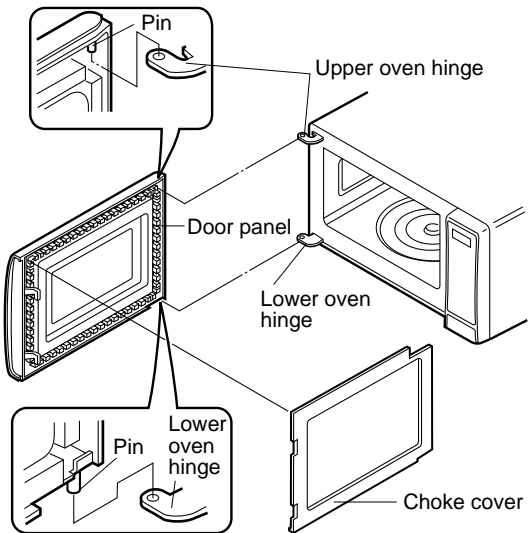
Figure C-8. Door Replacement
