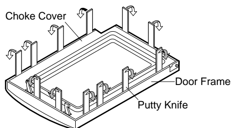
Figure C-7. Door Disassembly
