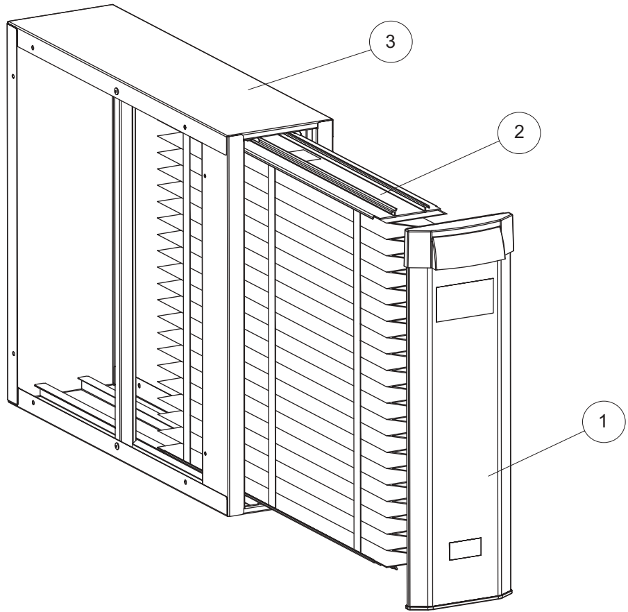
Figure 1: WHOLE HOUSE MERV 10 AND 13 AIR CLEANERS
