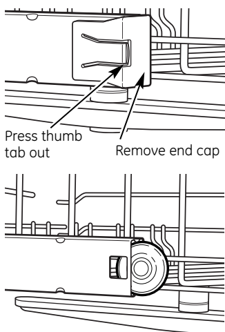
Shower Nozzle Service Part Number WD12X10134
