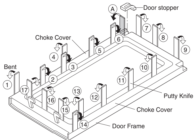
Figure C-3. Door Disassembly
