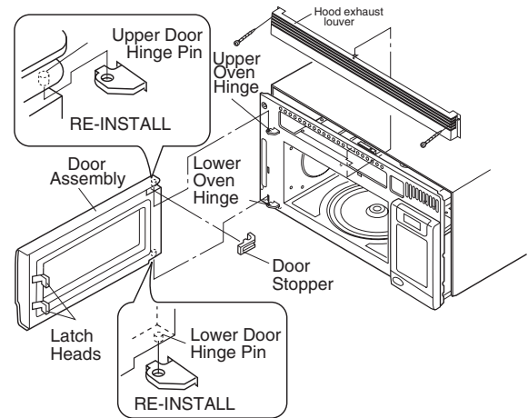
Figure C-2. Door Replacement and adjustment
