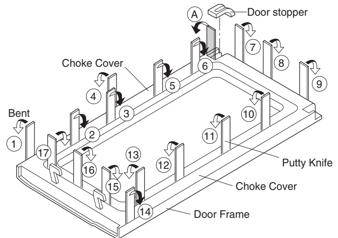
Figure C-3. Door Disassembly
