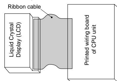
CPU unit
