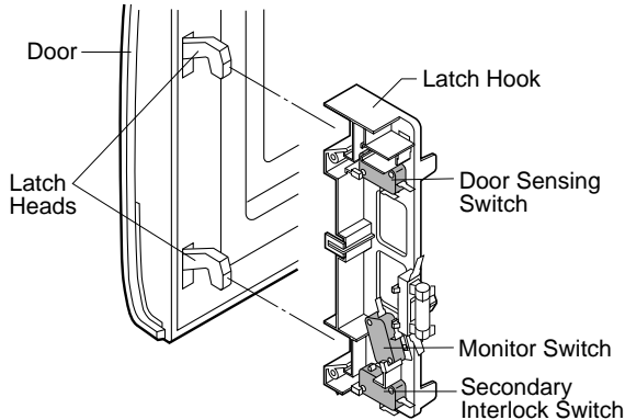
Figure D-1. Door Open Mechanism
