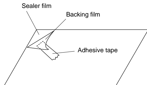
Figure C-6. Sealer film
