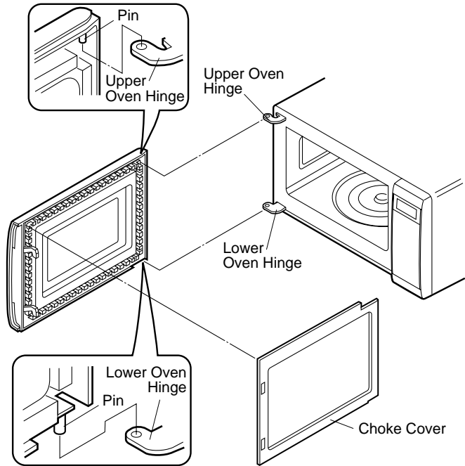
Figure C-5. Door Replacement
