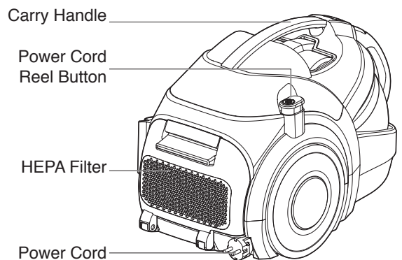
Power Cord
