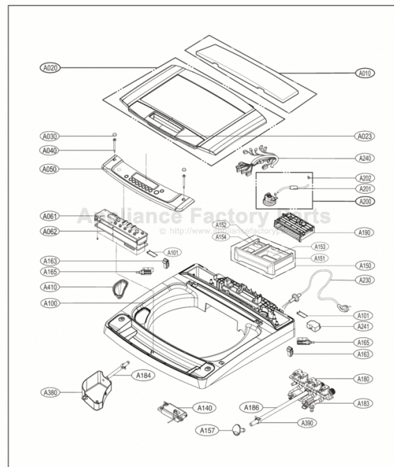
6-1. EXPLODED VIEW OF OUTER CASE ASSEMBLY
