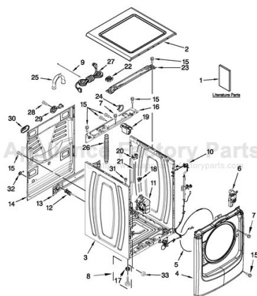
TOP AND CABINET PARTS
