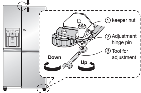
Height difference
