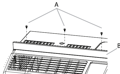
A. \frac{13}{32} " screws B. Top channel
