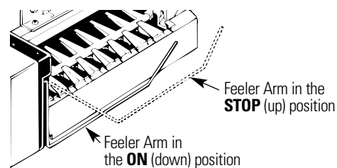
Feeler arm model
