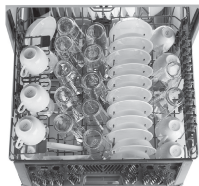
Upper Rack - 12 Place Settings - GDT530, GDF540 & GDT550
