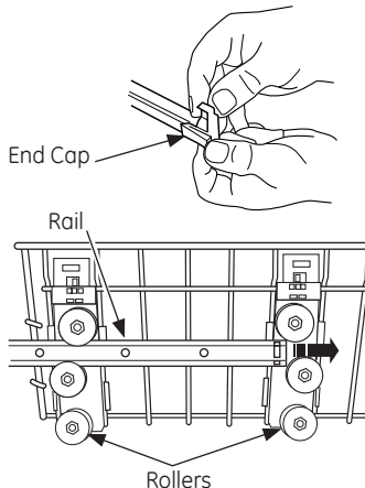
Upper Rack - 8 Place Settings - GDF510, GDF520 & ADT521
