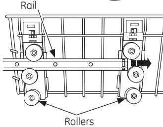
Upper Rack - 8 Place Settings - GDF510, GDF520 & ADT521
