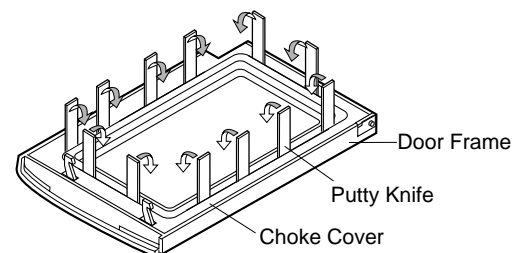
Figure C-4. Door Disassembly
