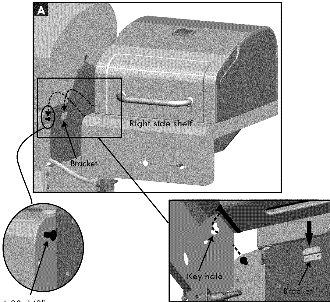
1/4-20x1/2" screw
