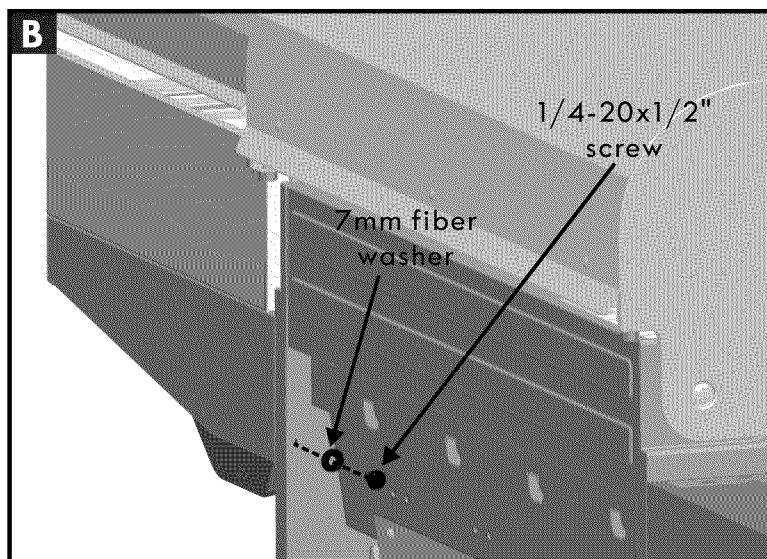
1/4-20x1/2" screw
