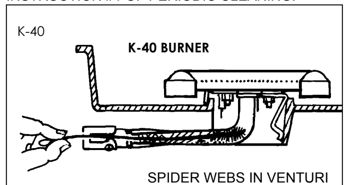
Figure 20 b Venturi cleaning out
