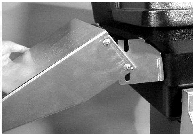
Figure 10 Hinging Shelf
