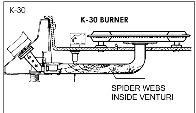
Figure 20 a Spider webs inside venturi
