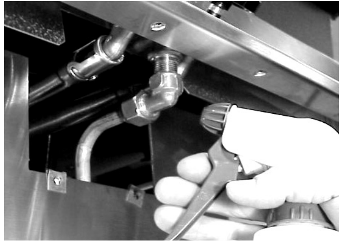
Figure 17 Leak Checking the Valve Connection
