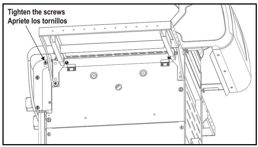
#8x3/8" self-tapping Screw Qty. 2 Tornillo autorroscante No. 8 de 3/8" Cant. 2
