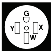
4-wire wall receptacle (14-50R) Figure 5A
