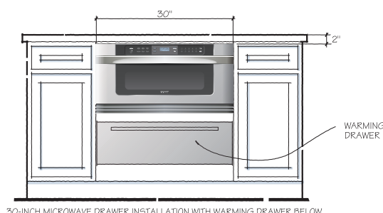
30-INCH MICROWAVE DRAWER INSTALLATION WITH WARMING DRAWER BELOW
