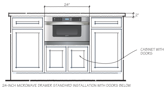
24-INCH MICROWAVE DRAWER STANDARD INSTALLATION WITH DOORS BELOW
