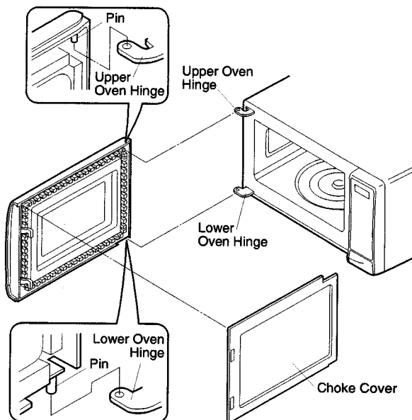
Figure C-5. Door Replacement
