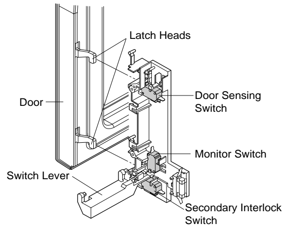
Figure C-3. Latch Switch Adjustments
