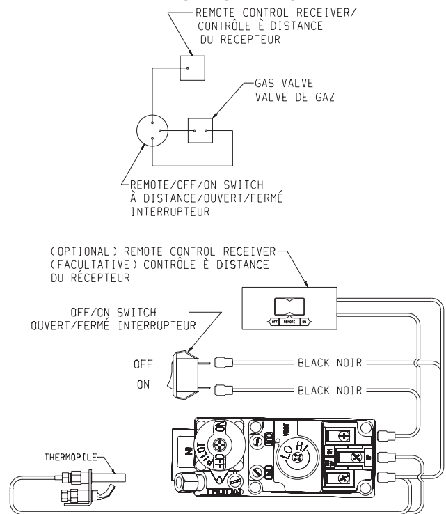
VSR Wiring Diagram (Figure 9)
