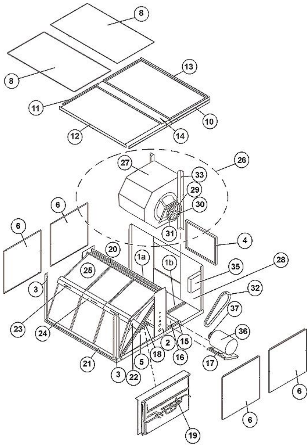
Exploded View 180-240
