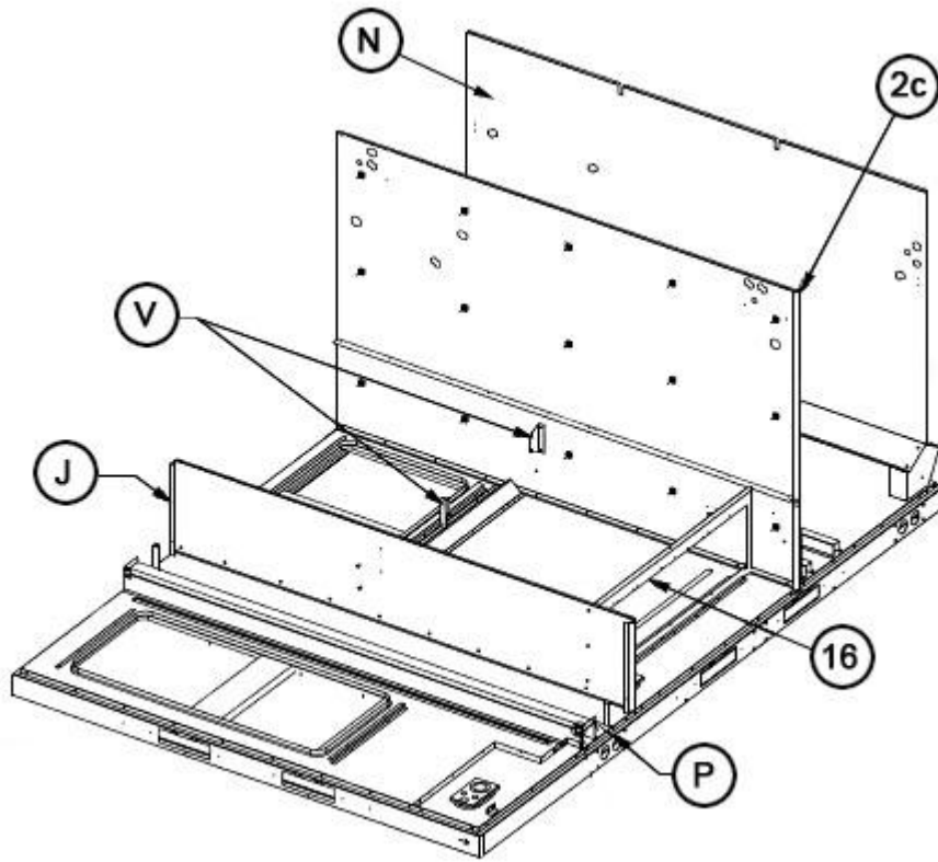
Heat Compartment 180-300
