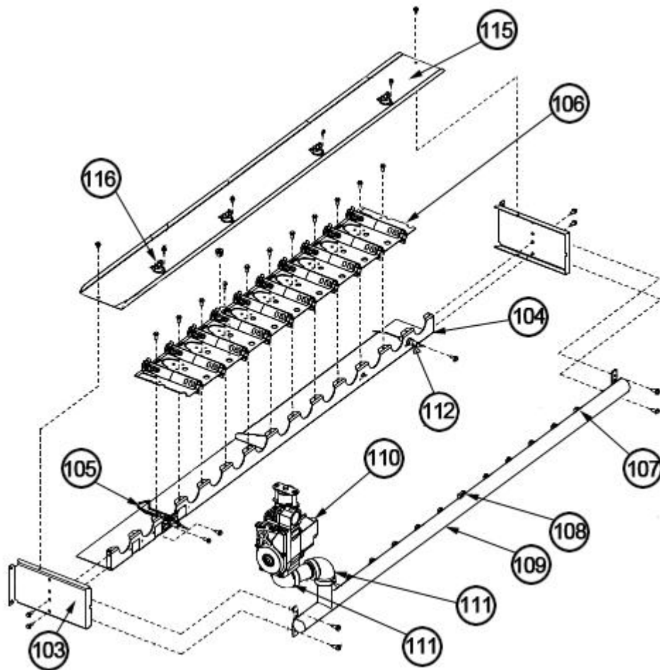
Burner Assembly 180-300
