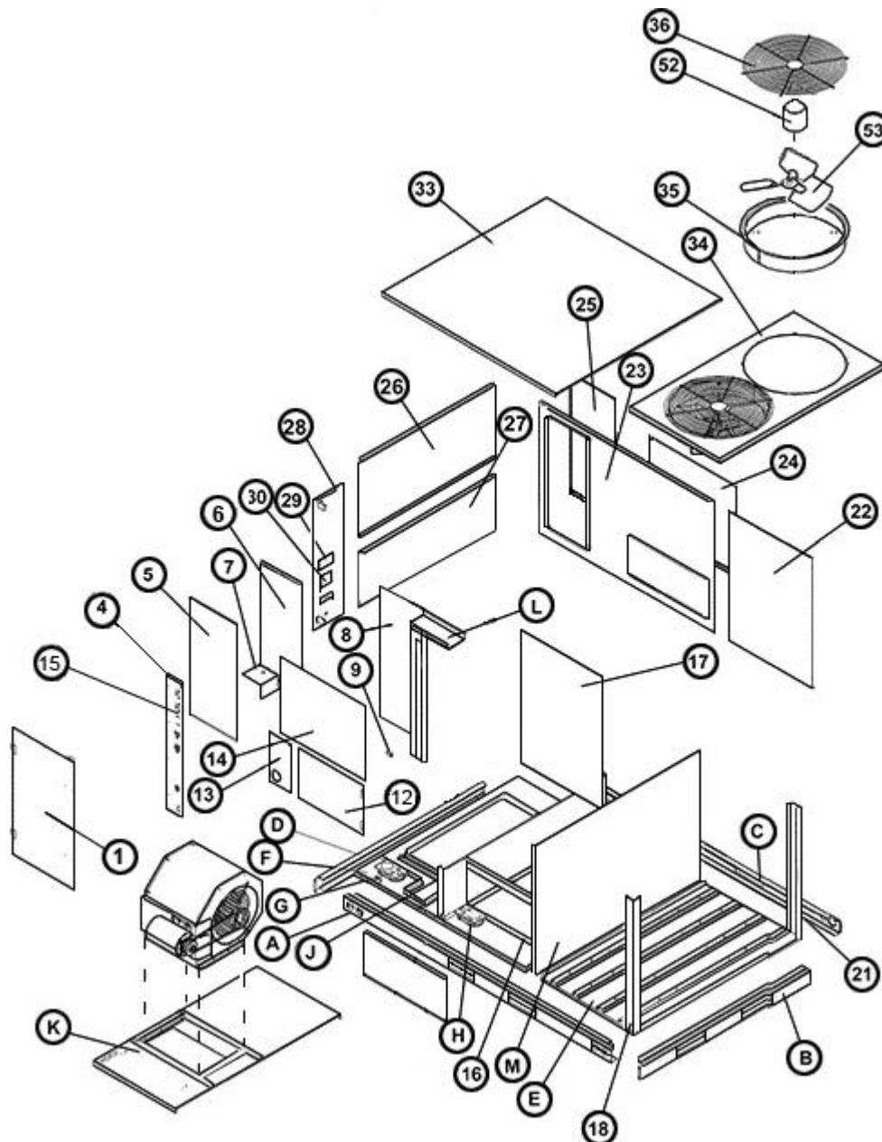
Exploded View 072-151
