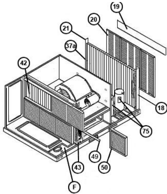
Filter-Coil Assembly 072-151
