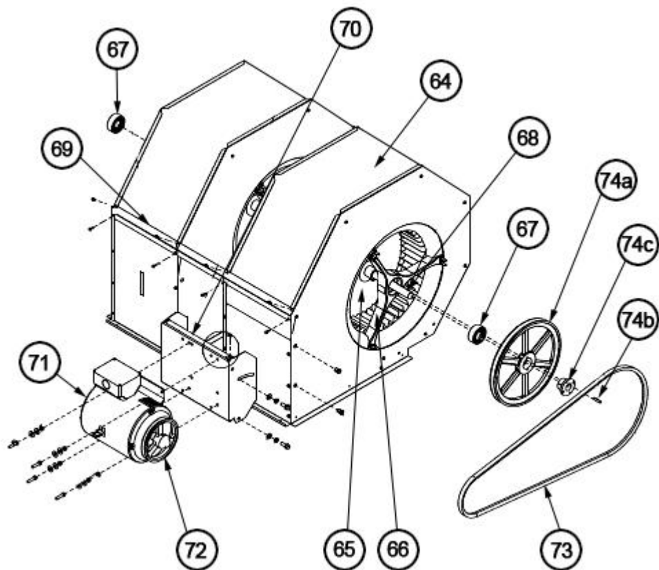
Blower Assembly 180-300
