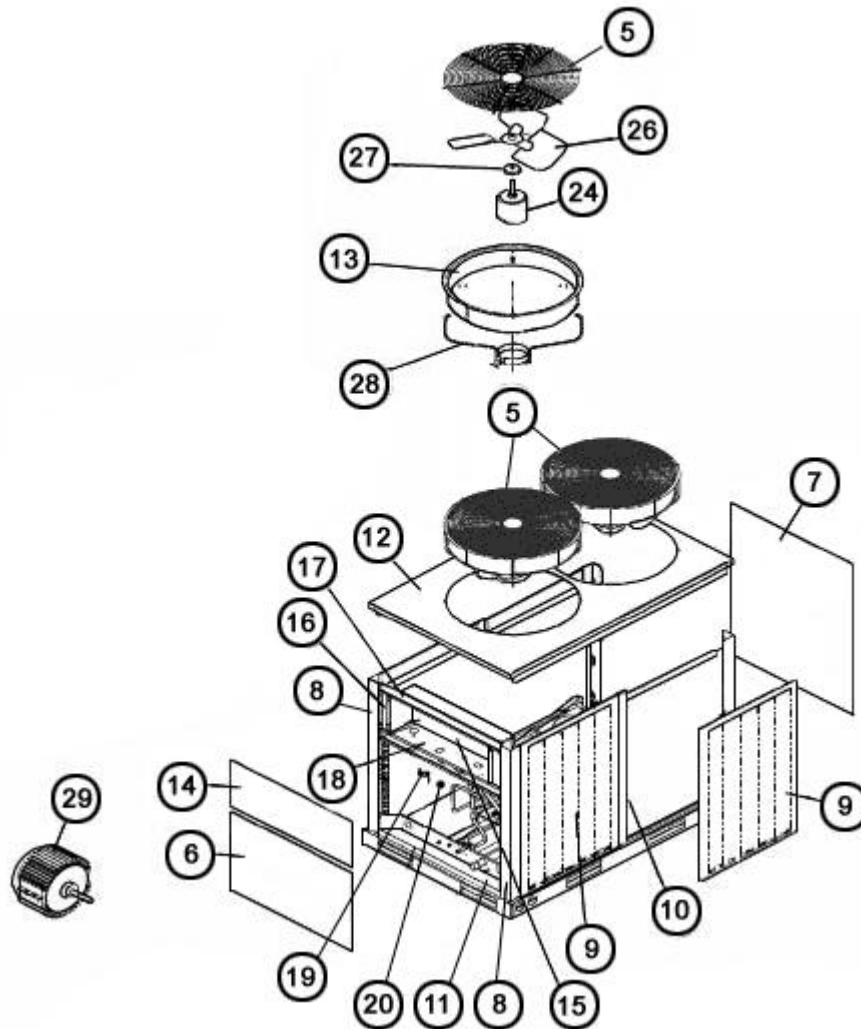
Exploded View 10-12
