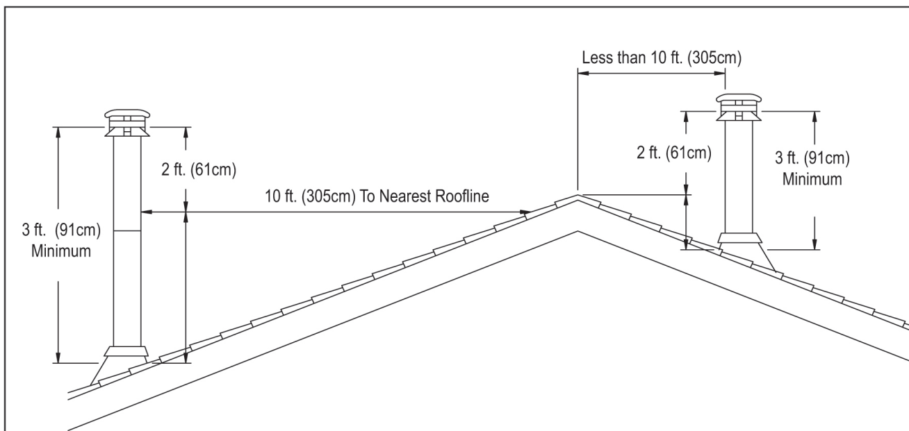
Pitched Roof
