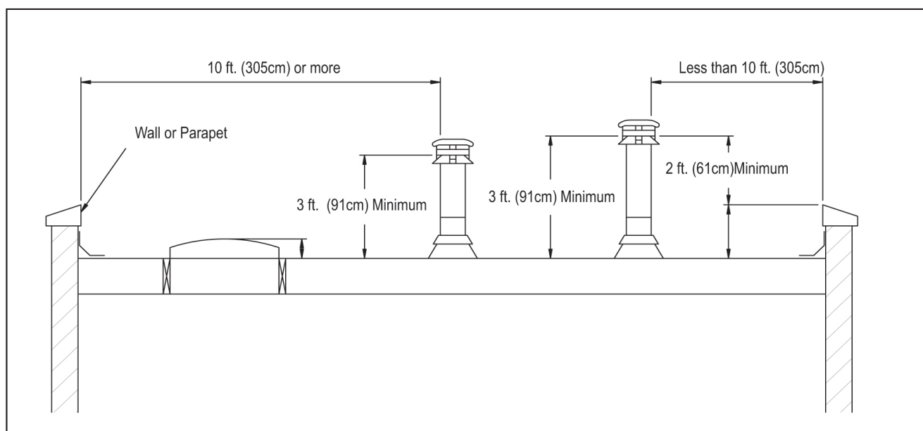
Flat Roof
