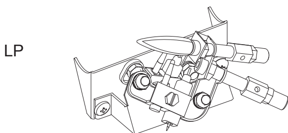
Fig. 20 - Correct Pilot Flame Pattern
