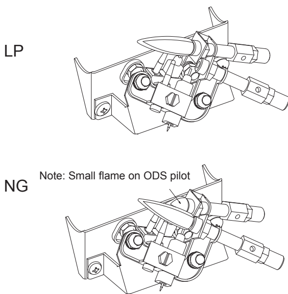
Fig. 20 - Correct Pilot Flame Pattern
