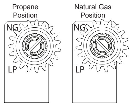
Fig. 8 - Selector Valve
