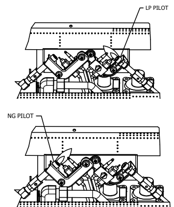
Fig. 16 - Pilot
