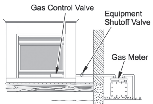
Fig. 8.2 - Checking Gas Joints (Natural Gas Only)
