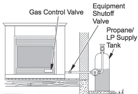
Fig. 8.1 - Checking Gas Joints (Propane/LP Only)
