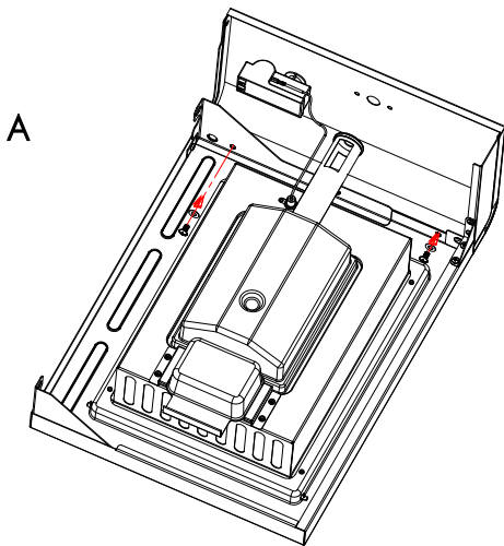
M6X13 screws Qty: 4 pcs
