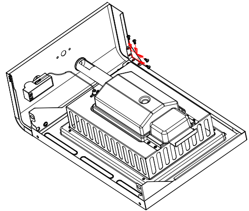
M6 compression washer Qty: 2 pcs
