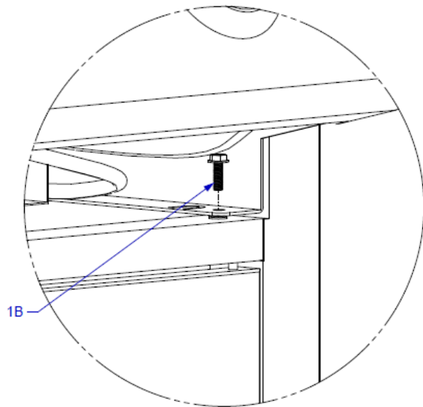
Detail C
