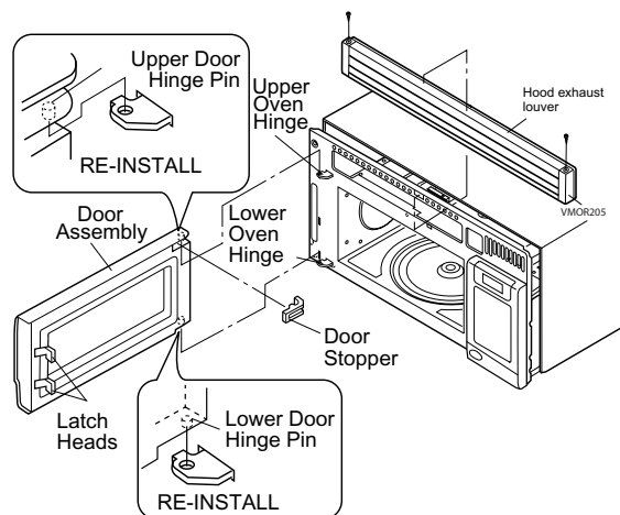
Figure C-2. Door Replacement and adjustment
