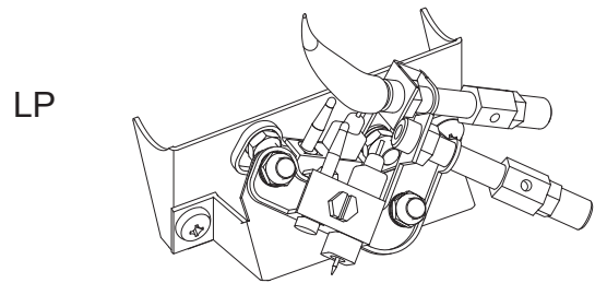
Fig. 21 - Incorrect Pilot Flame Pattern
