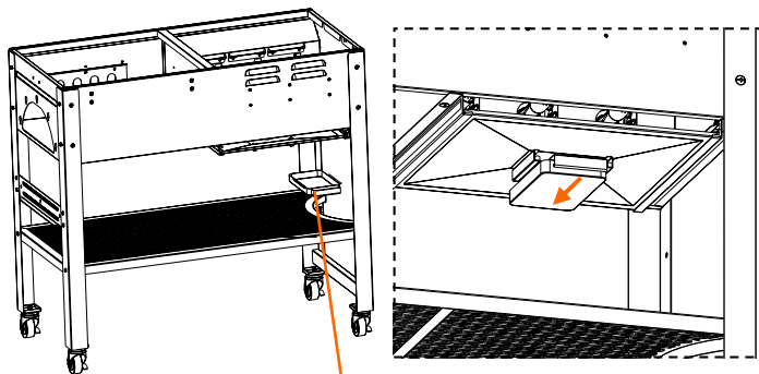
Fig. 7C Removable Grease Cup
