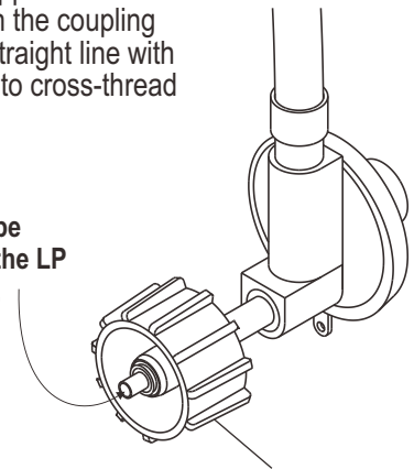
Coupling nut
